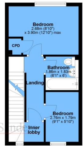
First Floor Approx. 29.1 sq. metres (312.7 sq. feet)
