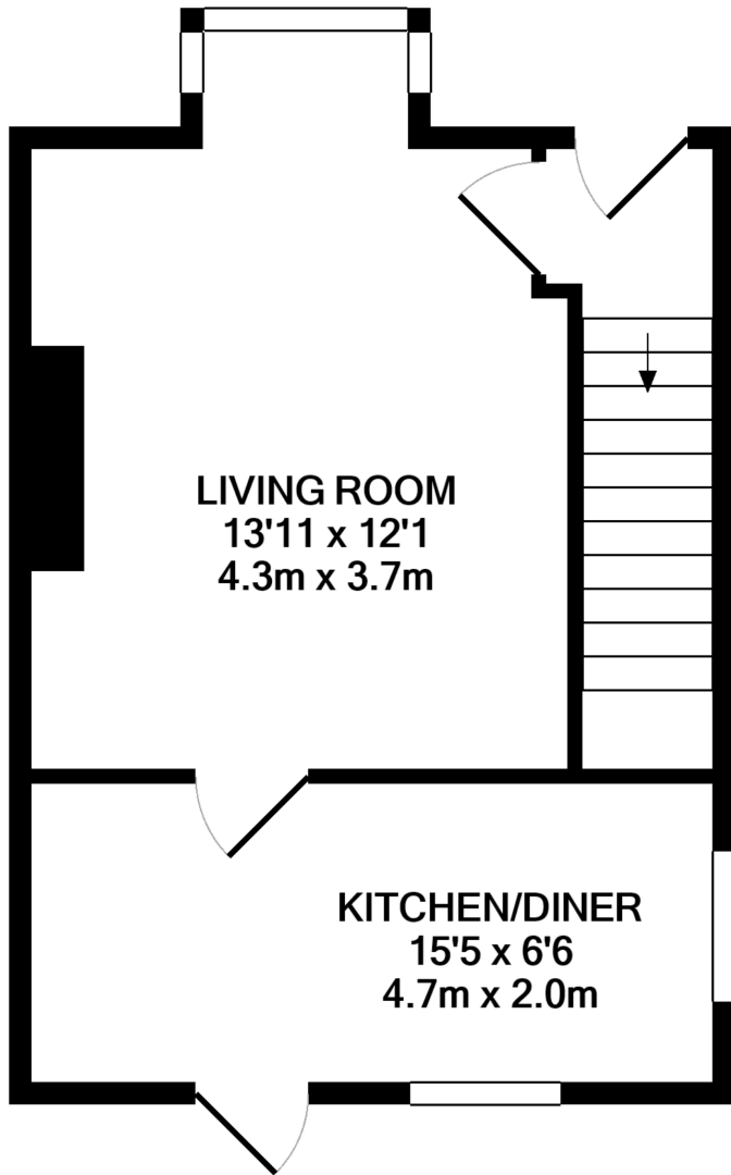
GROUND FLOOR APPROX. FLOOR AREA 326 SQ.FT. (30.3 SQ.M.)
