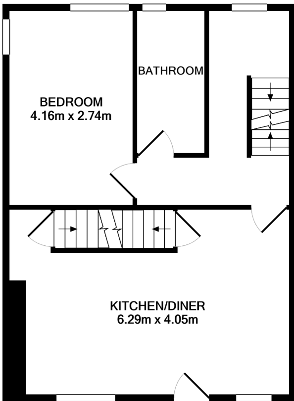
1ST FLOOR APPROX. FLOOR AREA 49.6 SQ.M. (534 SQ.FT.)
